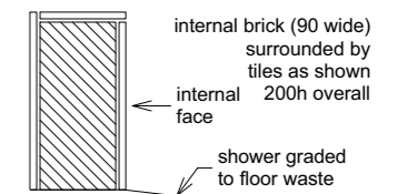
Tiled Hob Detail WAT1.2
