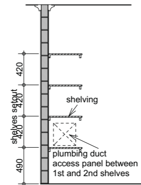
Plumbing duct access panel in Linen 1:50 DP1.1
