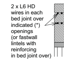
Opening HD Wires ET1.5 1:20
