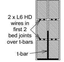
T-Bar HD Wires ET1.3 1:20
