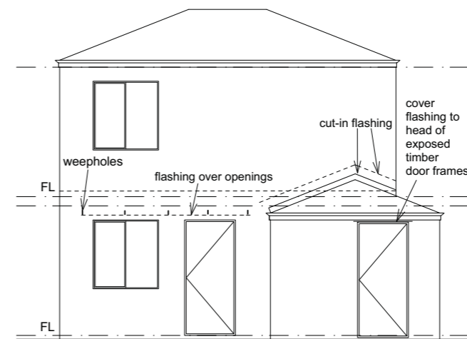
Sample Flashing Detail FS1.2
